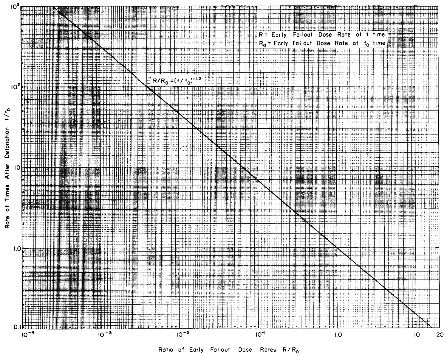
Fig. 2.18—Ratio of early fallout dose rates as a function of ratio of times after detonation.
